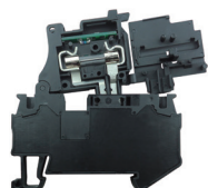
DST 4-HESILED24-D
